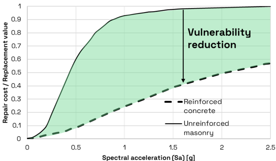
Figure 4. Vulnerability reduction: Vulnerability curves for a school facility built with unreinforced masonry (baseline) and with reinforced concrete (adapted). Adapted from: Rincón et al., 2017.
