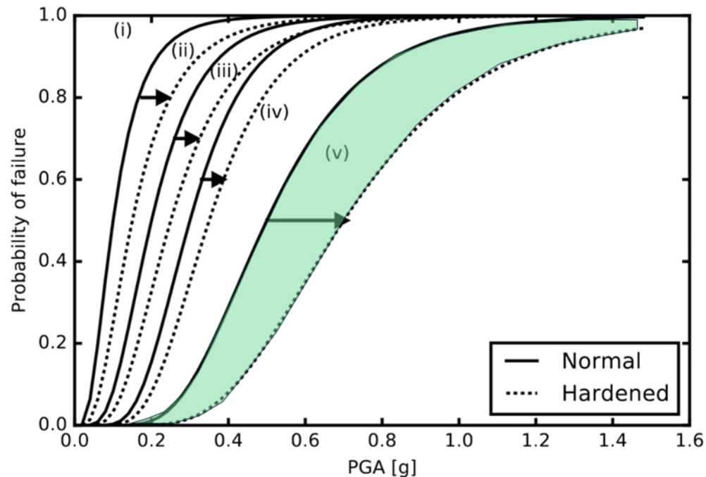
Figure 5. Vulnerability reduction: Fragility curves for an electrical substation with 5 damage states: (i) no damage, (ii) minor, (iii) moderate, (iv) extensive, and (v) complete damage, indicating curves for the normal and hardened cases. Adapted from: Lagos et al., 2020.
