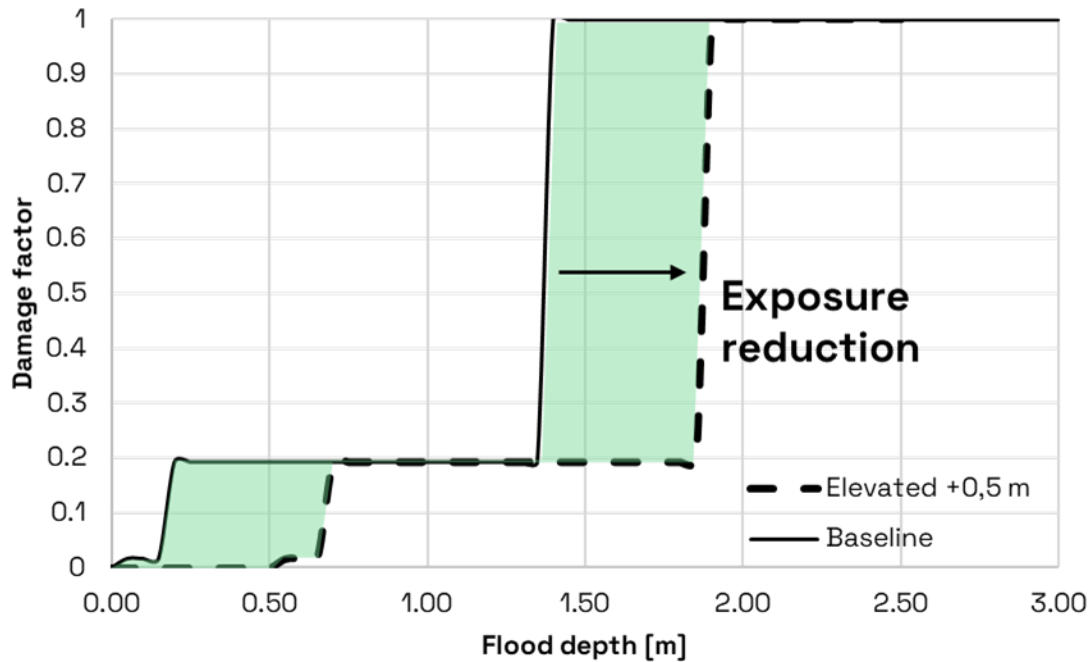
Figure 6. Exposure reduction: Vulnerability curve of rail infrastructure that has been elevated to reduce the exposure to flooding. Reproduced and adapted from: Kellermann et al., 2015.
